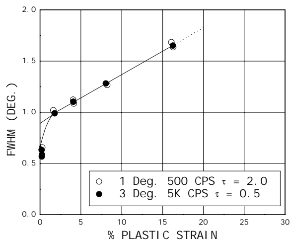
Fig. 3 - Inconel 600 Tubing, FWHM vs. Percent Plastic Strain CrK\alpha_{(311)} , 0.2 Deg. Receiving Slit Point Focus
