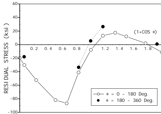
Fig. 10 - Longitudinal Residual Stress vs. (1+\cos \theta) Inconel 600, 2 1/2 % In. U-Bend
