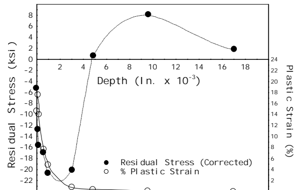
Fig. 5 - Longitudinal Residual Stress and Percent Plastic Strain, Ground Inconel 600 Tubing as Received
