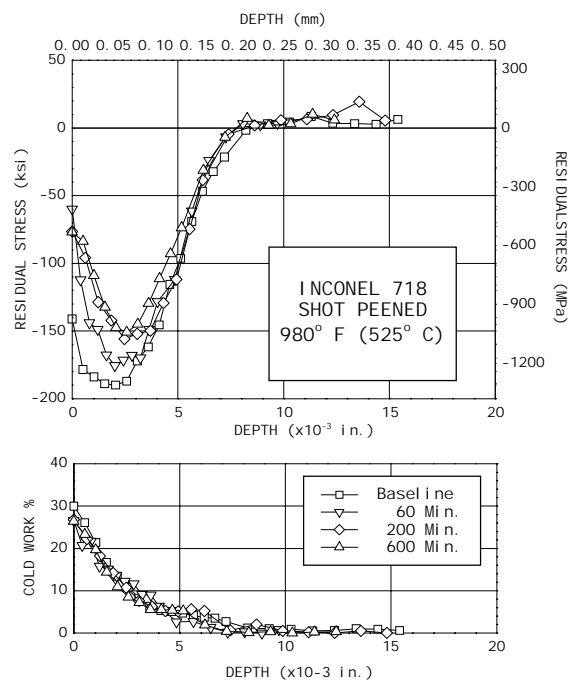
Fig. 6A – Thermal stress relaxation in shot peened Inconel 718 at 525 C (980 F).
