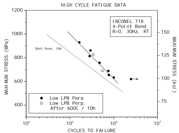
Figure 9 - Inconel 718, 4 point bend, R=0, 30Hz, RT.
