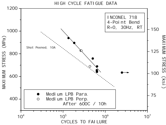
Figure 10 - Inconel 718, 4 point bend, R=0, 30 Hz, RT.
