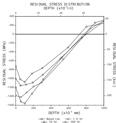
Figure 8 - Inconel 718 coupons. High LPB 600C.
