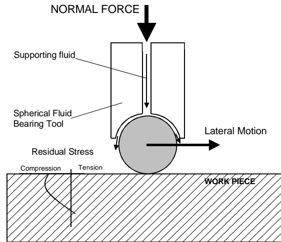
Figure 2 - Low Plasticity Burnishing schematic.
