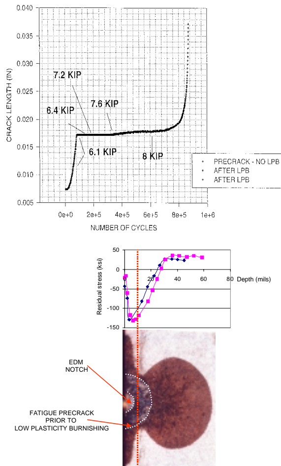
Figure 13. Effect of LPB on crack growth in E960 specimen precrack not removed.
