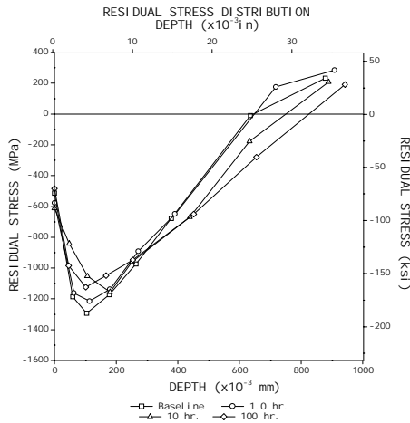
Figure 7 - Inconel 718 coupons. Medium LPB 600C.
