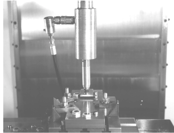
Figure 4 - LPB tool positioned for burnishing a coupon in a 20 HP vertical CNC mill.
