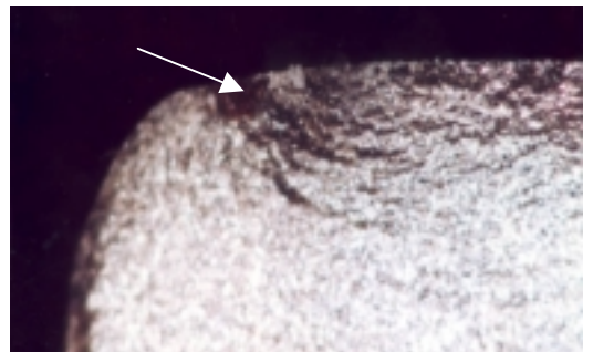
PRIMARY FAILURE INITIATED NEAR CORNER ADJACENT TO THE BURNISHED ZONE
