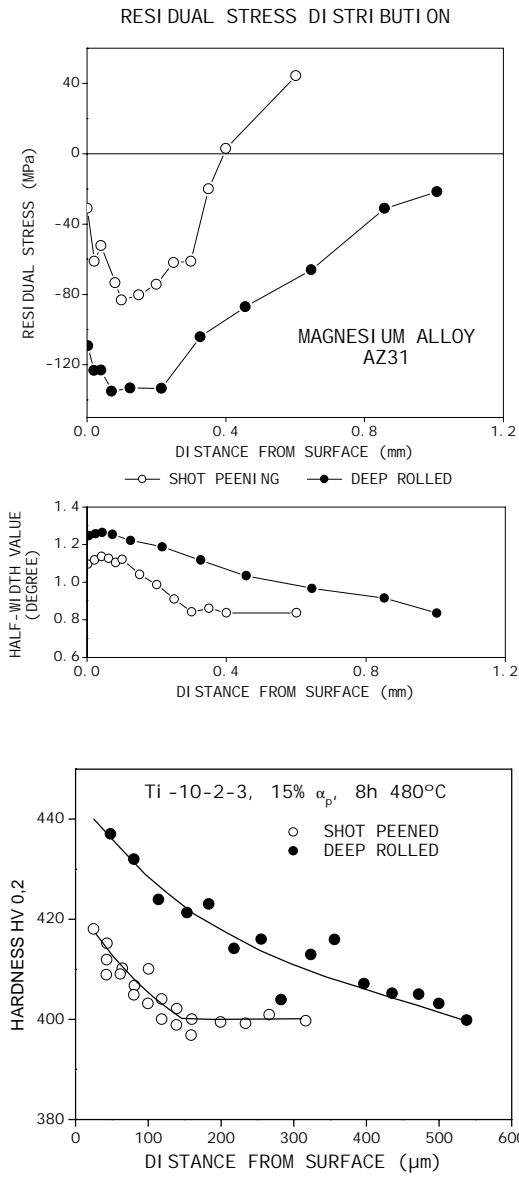
Figure 3 - a) Residual stress and peak width distributions produced by shot peening and deep rolling magnesium alloy AZ31, after Zinn and Scholtes [12], b) Micro hardness distributions produced by shot peening and deep rolling of Ti alloy Ti 10-2-3, after Drechsler... & Wagner [14].
