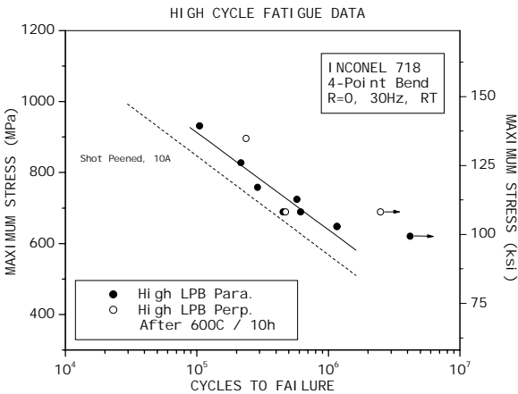
Figure 11 - Inconel 718, 4 point bend, R=0, 30 Hz, RT.
