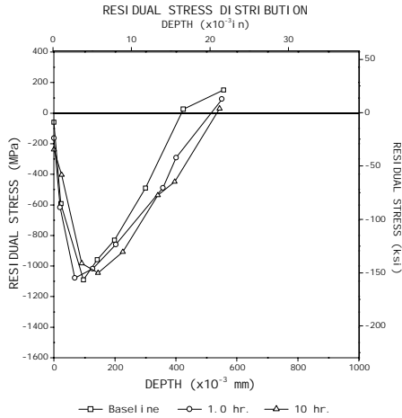
Figure 6 - Inconel 718 coupons. Low LPB 600C 10 hr.
