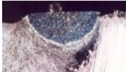
THE SIZE OF MONITORED CRACK IN THE DEPTH DIRECTION REACHED 0.022 IN. AT FAILURE
