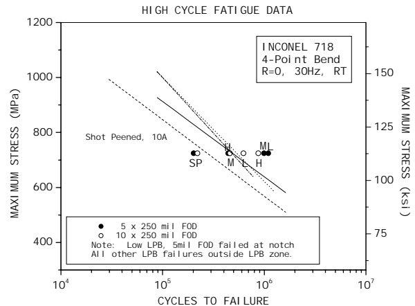
Figure 12 - Inconel 718, 4 point bend, R=0, 30Hz, RT.
