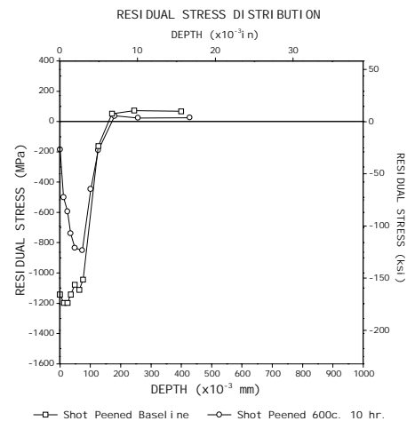
Figure 5 - Inconel 718 shot peened coupons. Baseline vs. thermal exposure at 600C 10 hr.
