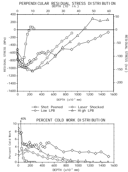
Figure 1 - Subsurface residual stress and cold work distributions produced by shot peening (8A), LSP (3X) and two levels of LPB in IN718.
