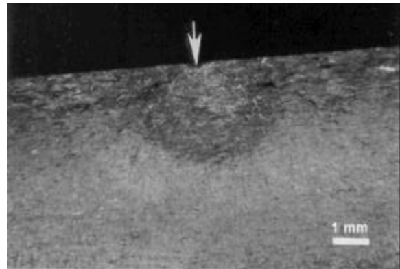
Figure 9 – Fatigue fracture surface of typical machined + 100hr salt fog exposure sample. Arrow indicates fatigue origin at the site of corrosion pit.
