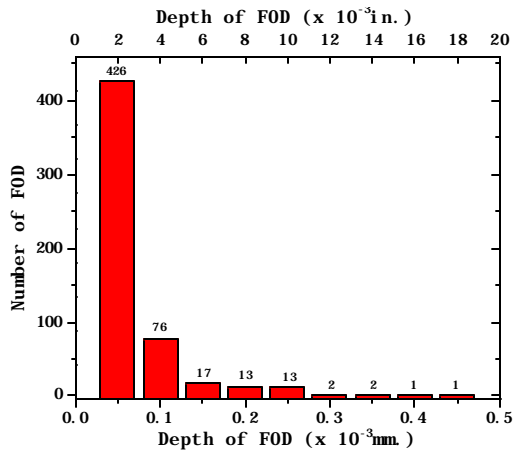
Figure 3 – Distribution of service generated FOD by depth regardless of position along the leading edge of the TI-6AL-4V first stage fan blade based upon ten (10) randomly used blades.
