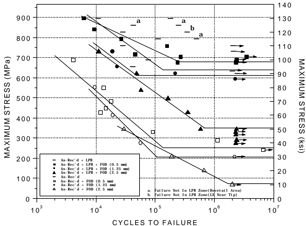
Figure 9 – S/N curves for the Ti-6Al-4V first stage fan blades as received (with service generated FOD) and with LPB for 0.5, 1.25 and 2.5 mm FOD.
