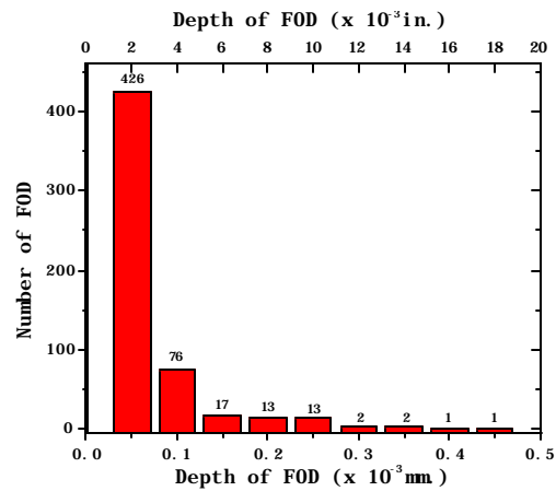
Figure 3 – Distribution of service generated FOD by depth regardless of position along the leading edge of the Ti-6Al-4V first stage fan blade based upon ten (10) randomly selected used blades.
