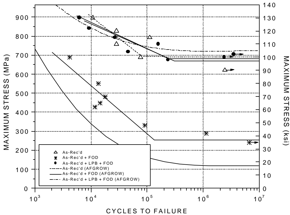
Figure 12 – Ti-6Al-4V first stage fan blade fatigue life predictions assuming -690 MPa ( -100 ksi) compression through the thickness with 0.5 mm FOD.
