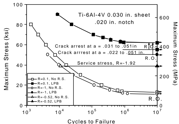
Figure 12 – HCF S-N curves calculated with AFGROW for 0.020 in. deep FOD and R-ratios of 0.1, -1.0 and -1.92 showing no significant effect of applied stress R-ratio with high residual compressive stress of -100 ksi.
