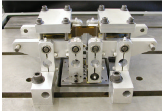
Figure 8 – Four-point bend fixture used for Ti-6-4 vane-edge feature samples, both single-edge ( R = 0.1 ) and double-edge ( R = -1 ), shown with a single-edge sample positioned for testing.
