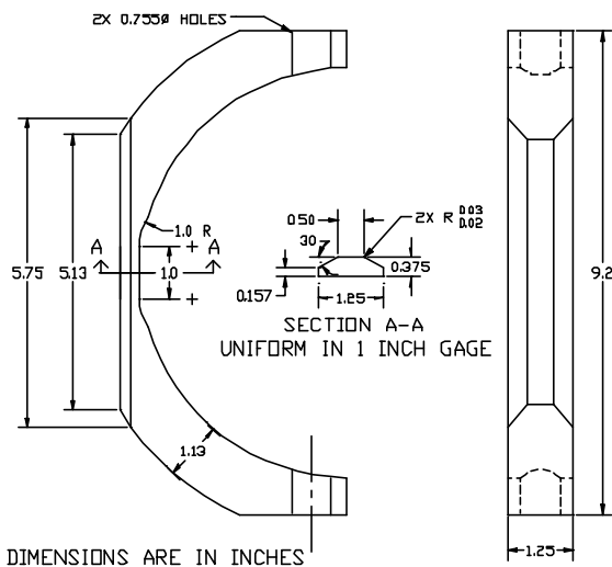
Figure 5 - C-ring specimen.
