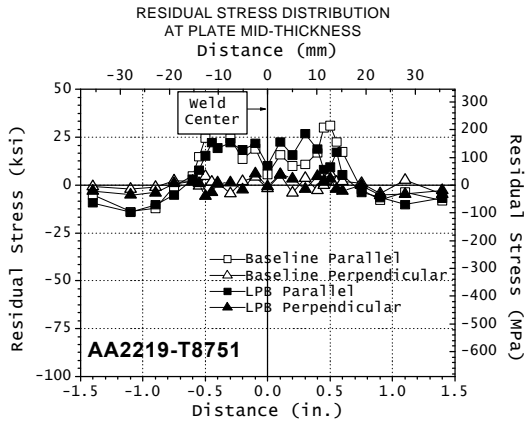
Figure 12 – Mid-thickness RS distribution in FSW AA2219-T8751
