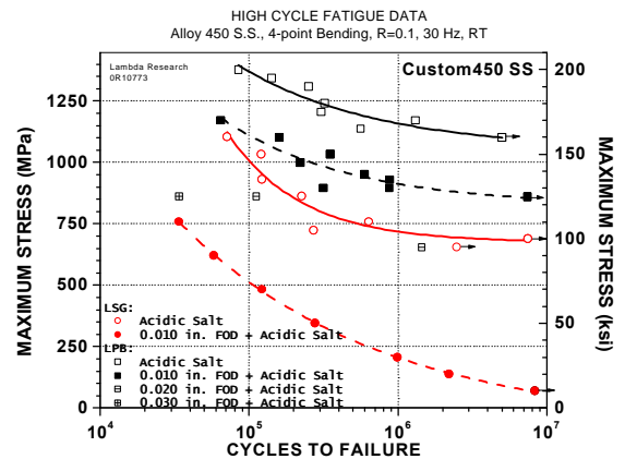
Figure 17 – S-N data for Custom 450 stainless steel.
