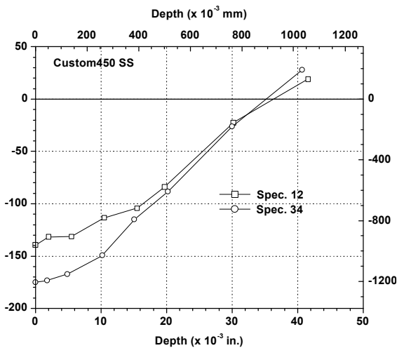
Figure 16 - Residual stress distribution for two LPB processed (and fatigue tested) specimens. Specimen #12 (LPB - no notch): Smax = 195 ksi (~1,345 MPa); Nf = 141,191 cycles. Specimen #34 (LPB + notch): Smax = 160 ksi (~1,100 MPa); Nf = 159,941 cycles
