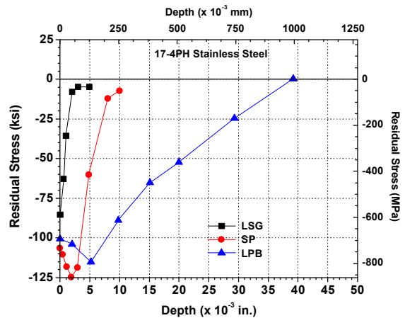
Figure 14 – RS profiles for surface treated 17-4PH SS
