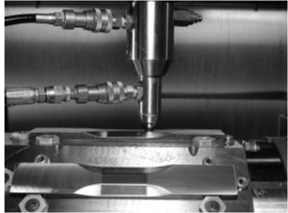
Figure 2 – LPB processing of fatigue samples with at single point contact LPB tool in a 4-axis CNC mill.
