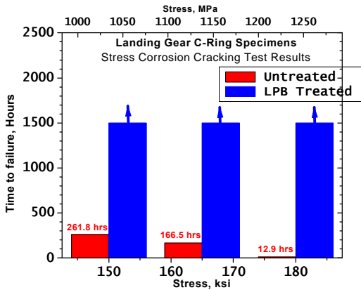
Figure 8 – SCC test results for 300M Steel
