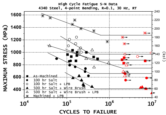
Figure 4 – S-N plots of salt fog exposed 4340 steel.
