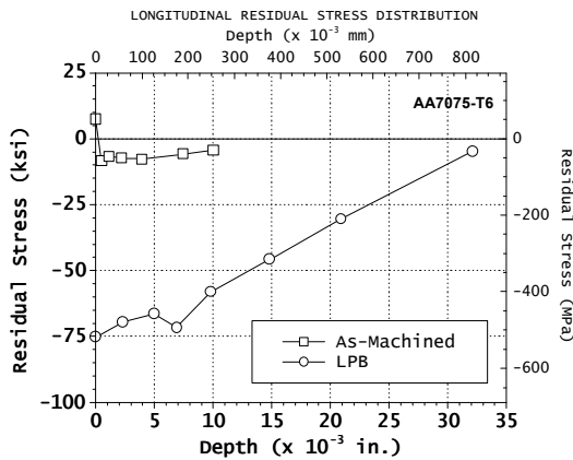
Figure 9 – RS distribution in AA7075-T6
